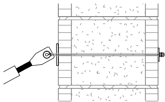
CMU with Thru Bolt
