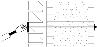
Brick/Block with Thru Bolt
