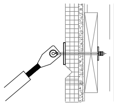
EIFS with Thru Bolt
