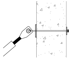
Tilt Up Wall with Thru Bolt
